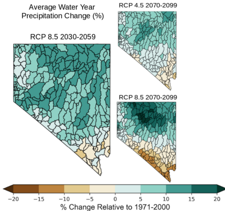
Fig. X.5. Average percent change in annual precipitation for the near-term (2030-2059, left) and the late 21 st century under lower (RCP4.5, upper right) and higher (RCP8.5, lower right) emissions scenarios. Source: Nevada Climate Initiative https://climateaction.nv.gov/policies/climate-nv
