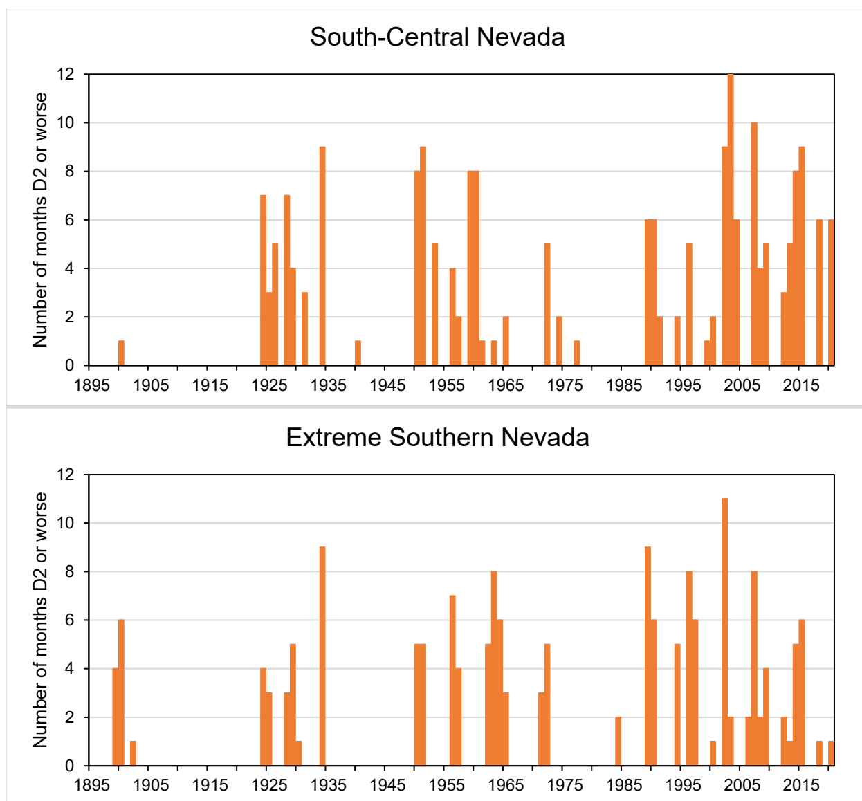
Figure X.3. Number of months per year when each climate division in Nevada experienced drought equivalent to the US Drought Monitor's D2 – Severe Drought or worse based on the Palmer Drought Severity Index (PDSI). According to US Drought Monitor guidance, PDSI < -3 indicates D2 or worse drought. Monthly PDSI from NOAA National Centers for Environmental information, Climate at a Glance (retrieved November 23, 2021). https://www.ncdc.noaa.gov/cag/
