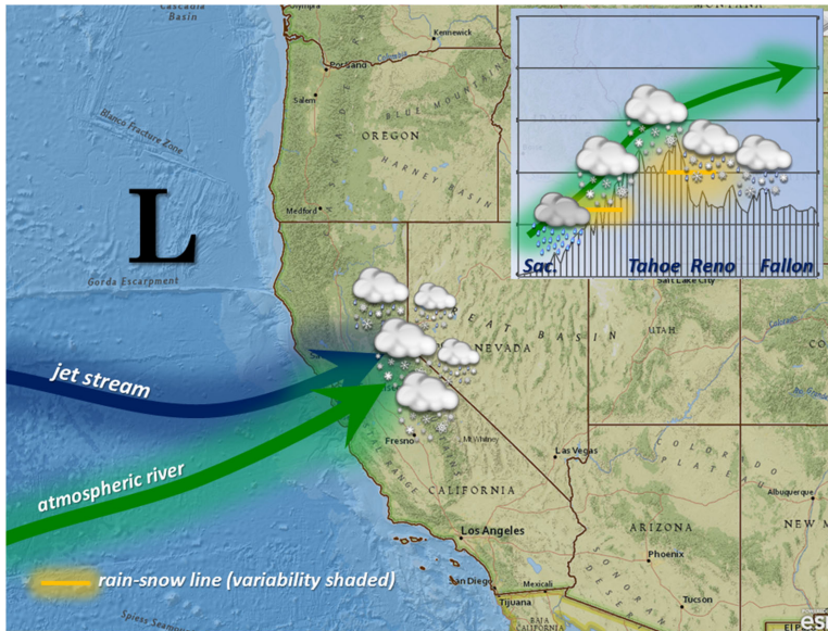
Figure 3-39. Schematic showing a classic weather pattern for heavy snows in central and northern Nevada of the patterns for heavy snows in northern and central Nevada – a cold atmospheric river scenario.
