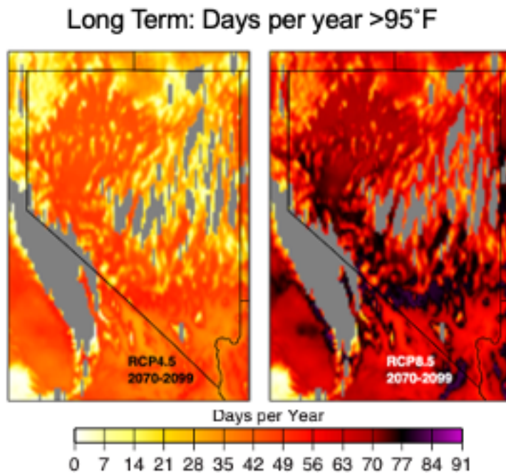
Figure X.3. Long-term increase in number of days per year in the when daytime high temperatures will exceed 95°F under a low emissions scenario (RCP4.5, left) and a high emissions scenario (RCP8.5, right). Source: Nevada Climate Strategy. Climate Change in Nevada. https://climateaction.nv.gov/policies/climate-nv/
