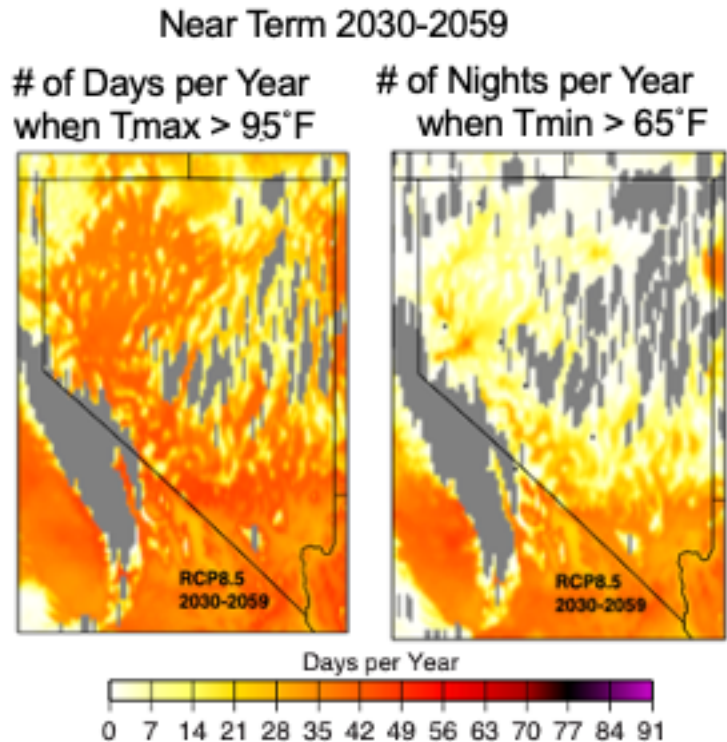
Figure X.2. Near-term increase in number of days per year in the when daytime high temperatures will exceed 95°F (left) and when nighttime temperatures will remain above 65°F. Both use the RCP8.5 emissions scenario. This is higher emissions scenario in the long-term, similar to the RCP4.5 scenario in the near-term. Source: Nevada Climate Strategy. Climate Change in Nevada. https://climateaction.nv.gov/policies/climate-nv/
