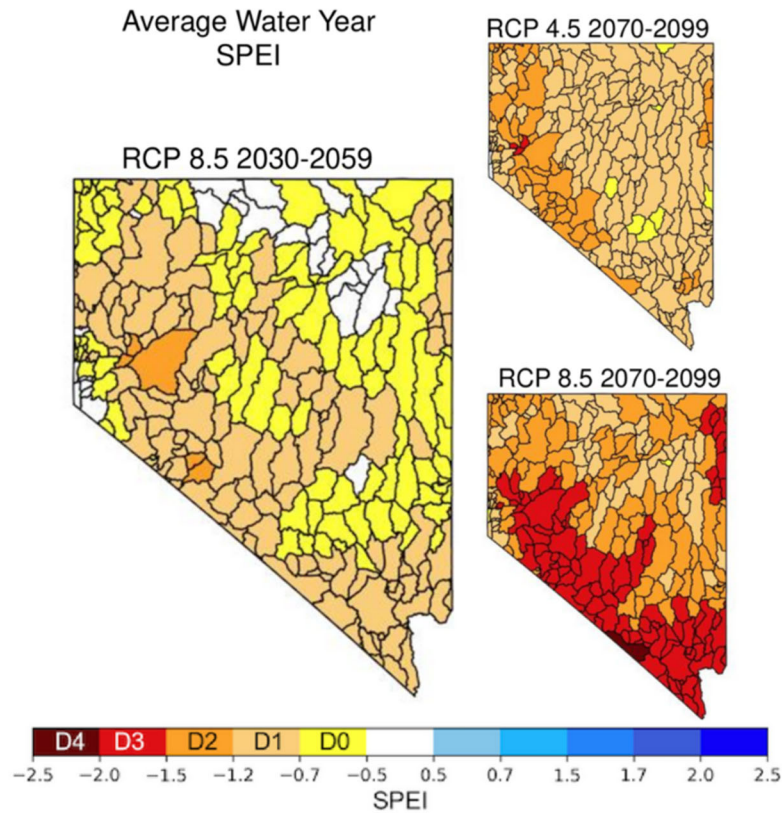
Fig. X.4. Drought conditions tracked by the Standardized Precipitation – Evaporation Index (SPEI), a drought index that, like the Palmer Drought Severity Index, tracks both precipitation and temperature effects on drought. Conditions are shown for the near-term (2030-2059, left) and the late 21 st century under lower (RCP4.5, upper right) and higher (RCP8.5, lower right) emissions scenarios. Source: Nevada Climate Initiative https://climateaction.nv.gov/policies/climate-nv
